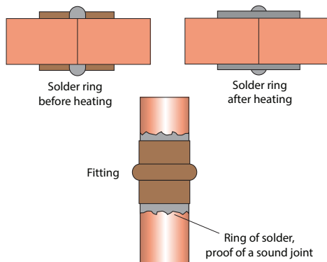
Figure 2: Solder ring fitting
